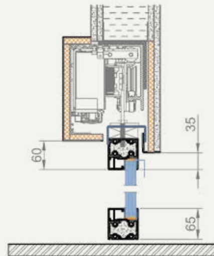
Vertical cross-section
